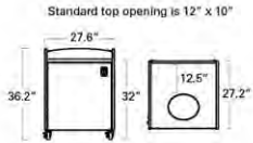
WR18-20 WASTE RECEPTACLE
