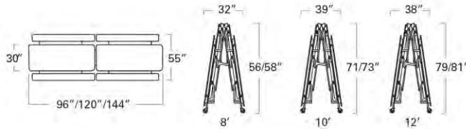
59TV BENCH TABLE - 8', 10', 12' (27"/29" high)
