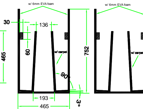
B-B VIEW
