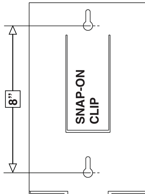
1 Box Mounting Dimensions
