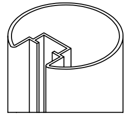
4" O.D. ROUND EXTRUDED ALUMINUM
