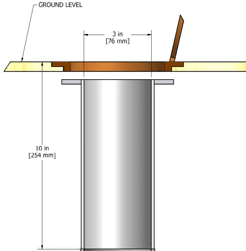
Figure 3-1: Correct Ground Sleeve Dimensions
