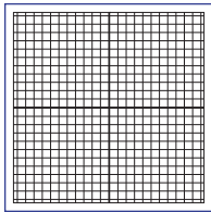
Graph Coordinates
